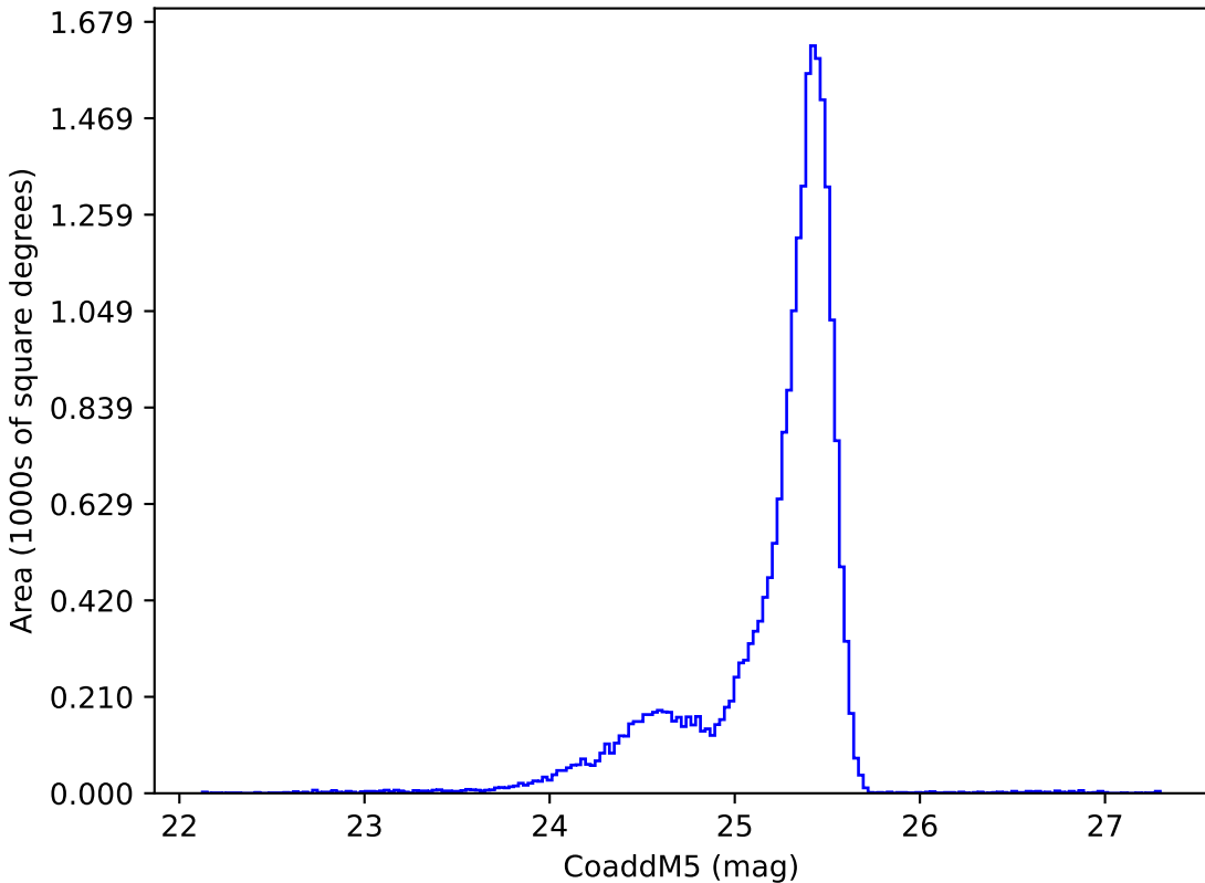
roll_pause_mjdp270_v3.4_10yrs u: CoaddM5
