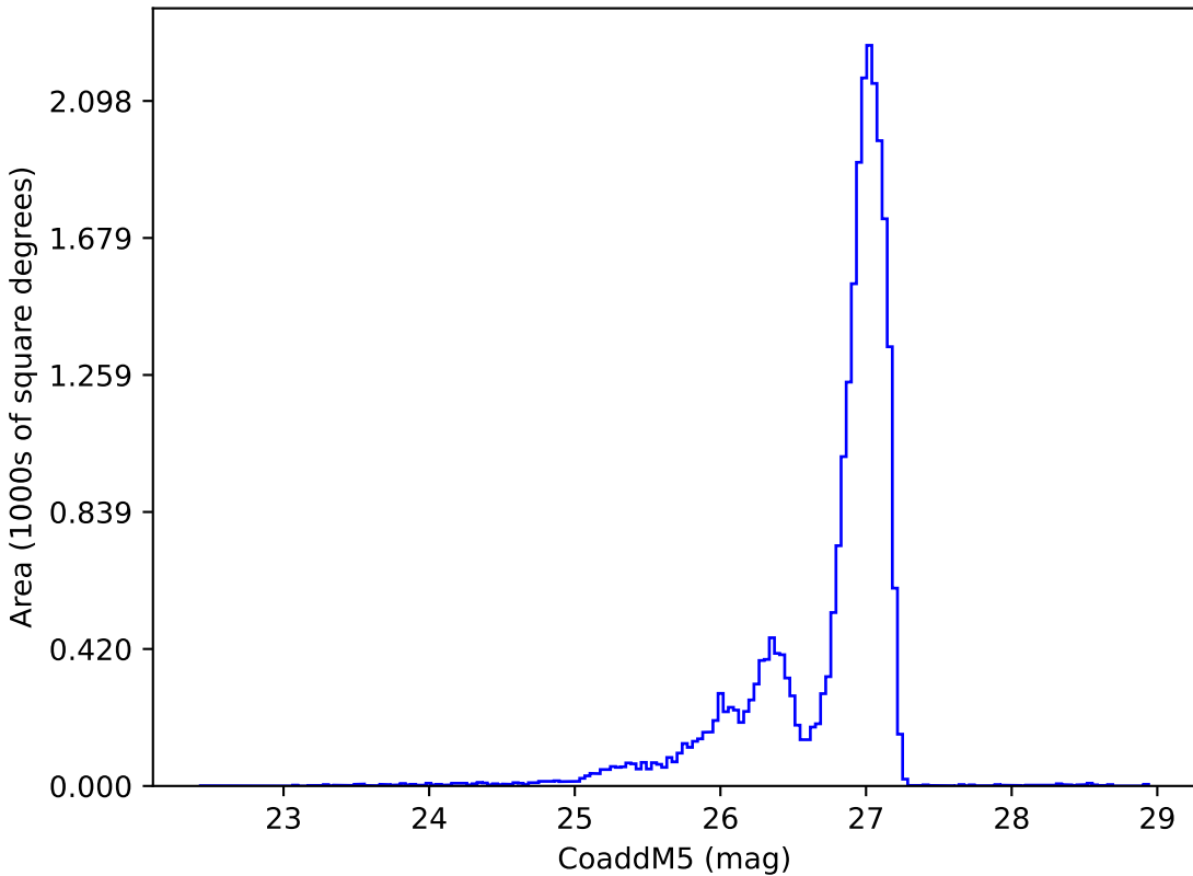
roll_pause_mjdp270_v3.4_10yrs r: CoaddM5
