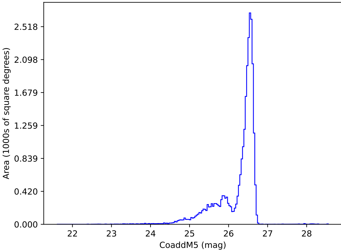
roll_pause_mjdp270_v3.4_10yrs i: CoaddM5
