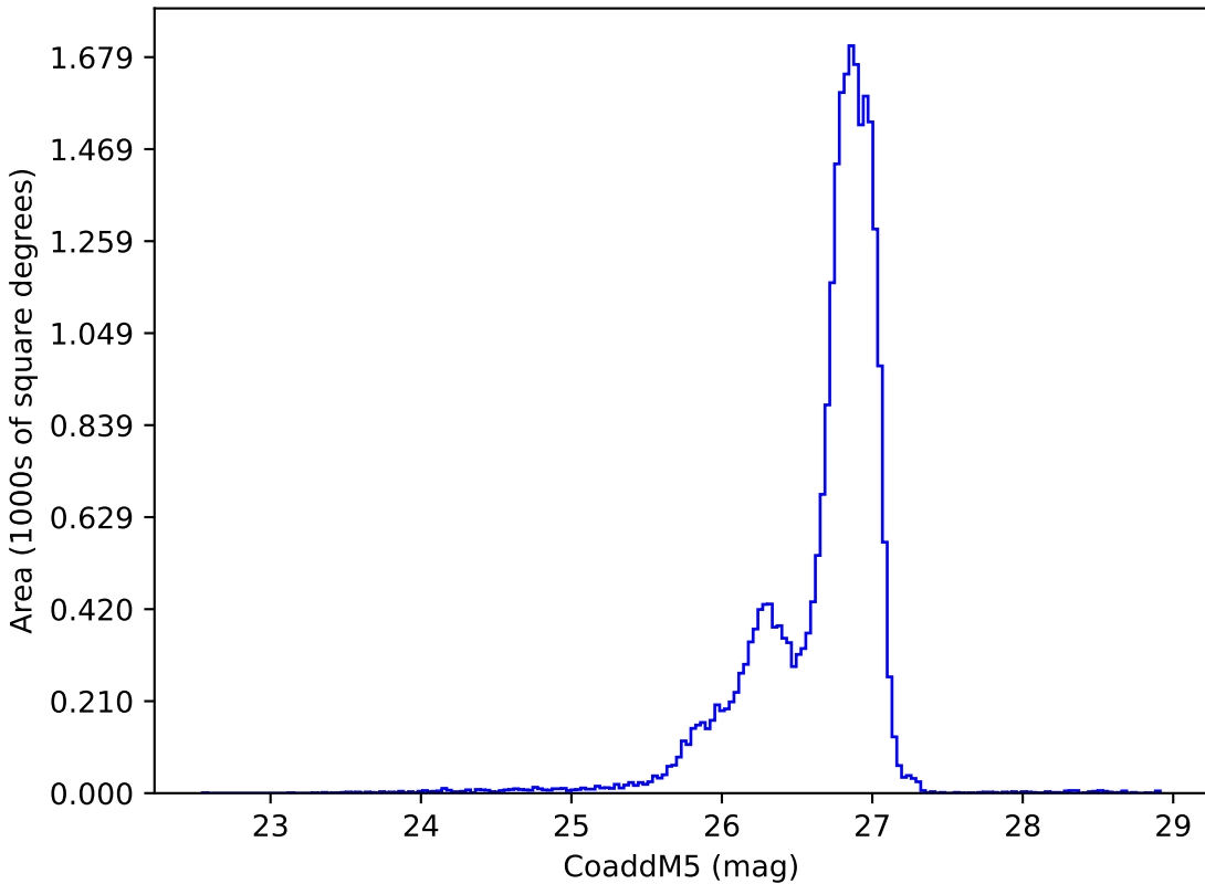
roll_pause_mjdp270_v3.4_10yrs g: CoaddM5
