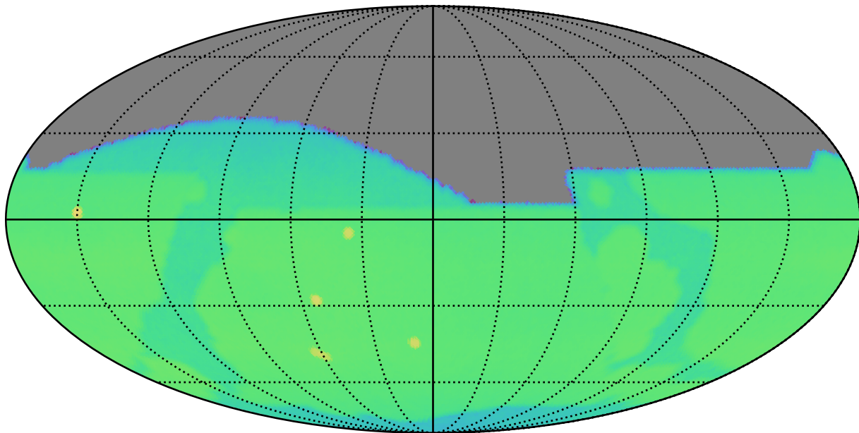
roll_pause_mjdp270_v3.4_10yrs : CoaddM5
