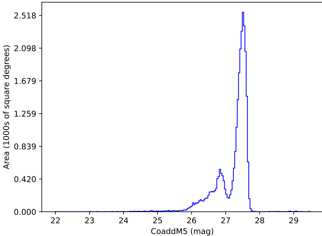
roll_pause_mjdp270_v3.4_10yrs : CoaddM5
