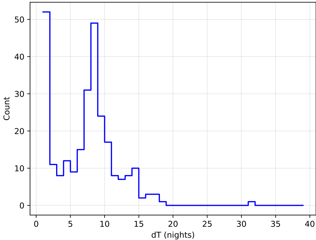
roll_pause_mjdp270_v3.4_10yrs all bands: DD:XMM_LSS Delta Nights Histogram
