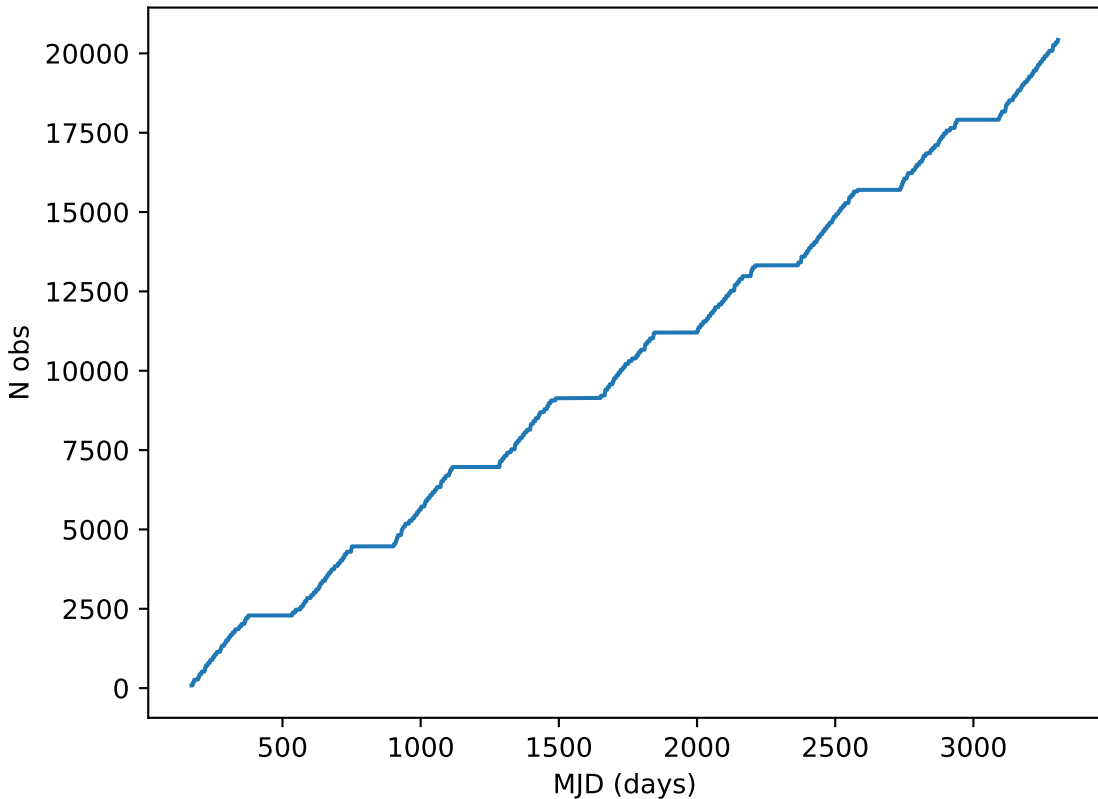
roll_pause_mjdp270_v3.4_10yrs all bands: DD:XMM_LSS Cumulative NVisits
