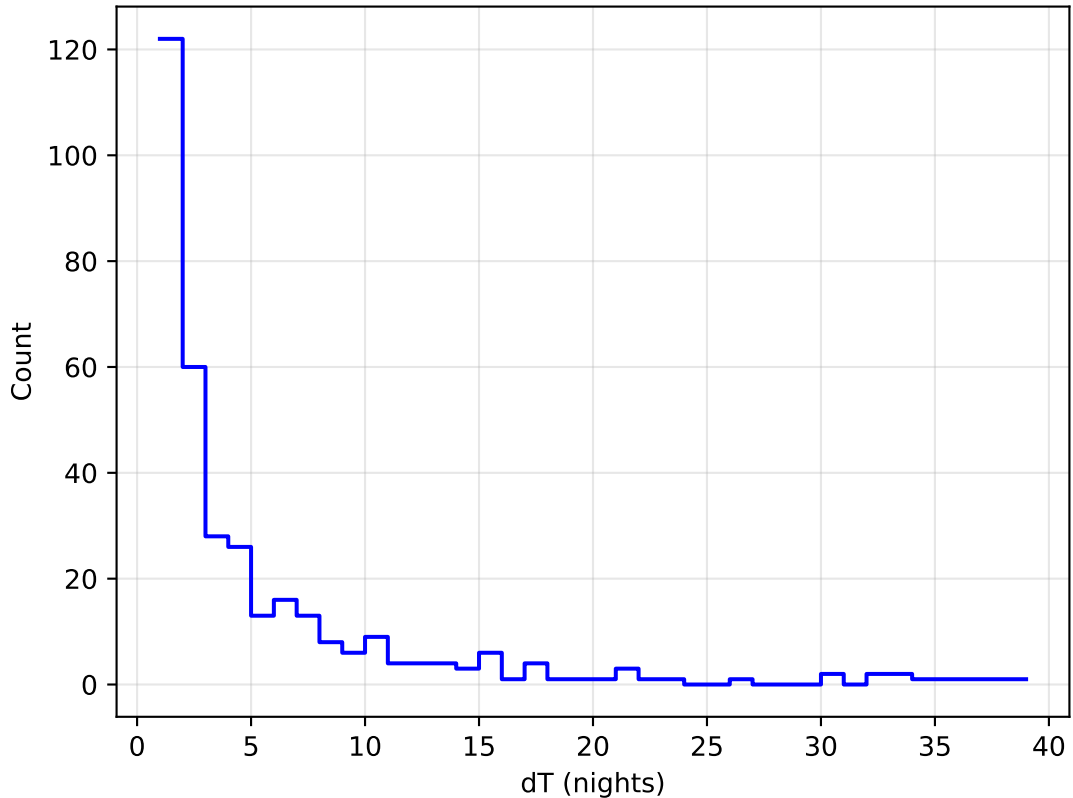
roll_pause_mjdp270_v3.4_10yrs all bands: DD:WFD Delta Nights Histogram
