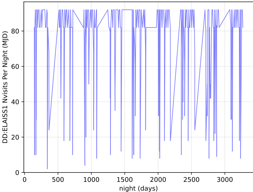
roll_pause_mjdp270_v3.4_10yrs all bands: DD:ELAISS1 Nvisits Per Night
