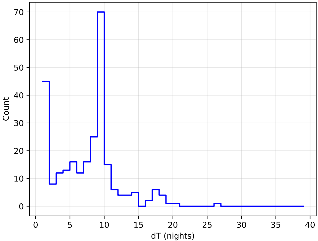
roll_pause_mjdp270_v3.4_10yrs all bands: DD:ELAISS1 Delta Nights Histogram
