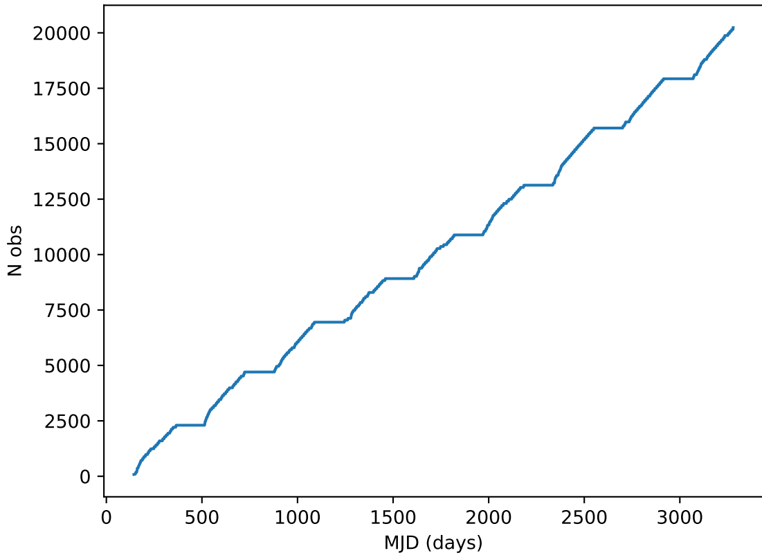
roll_pause_mjdp270_v3.4_10yrs all bands: DD:ELAISS1 Cumulative NVisits
