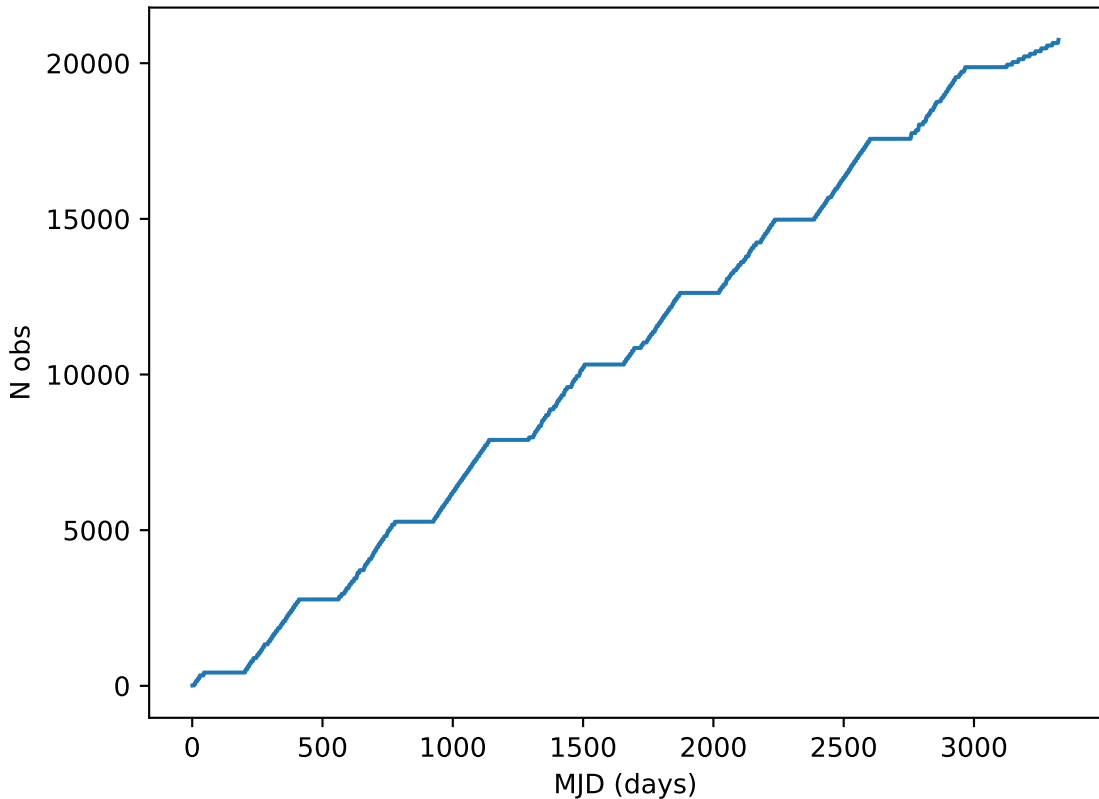
roll_pause_mjdp270_v3.4_10yrs all bands: DD:EDFS Cumulative NVisits
