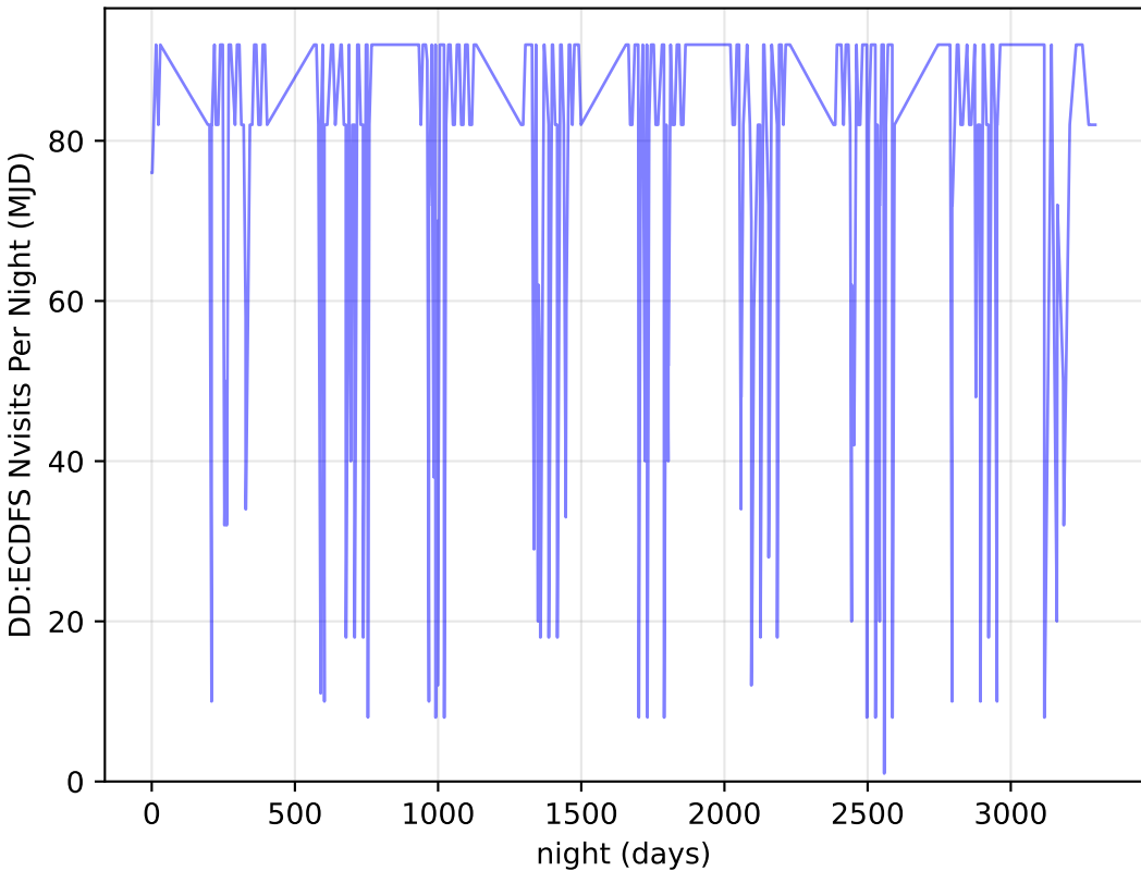
roll_pause_mjdp270_v3.4_10yrs all bands: DD:ECDFS Nvisits Per Night
