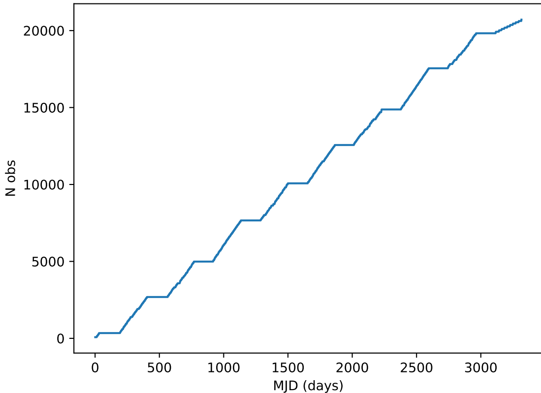
roll_pause_mjdp270_v3.4_10yrs all bands: DD:ECDFS Cumulative NVisits
