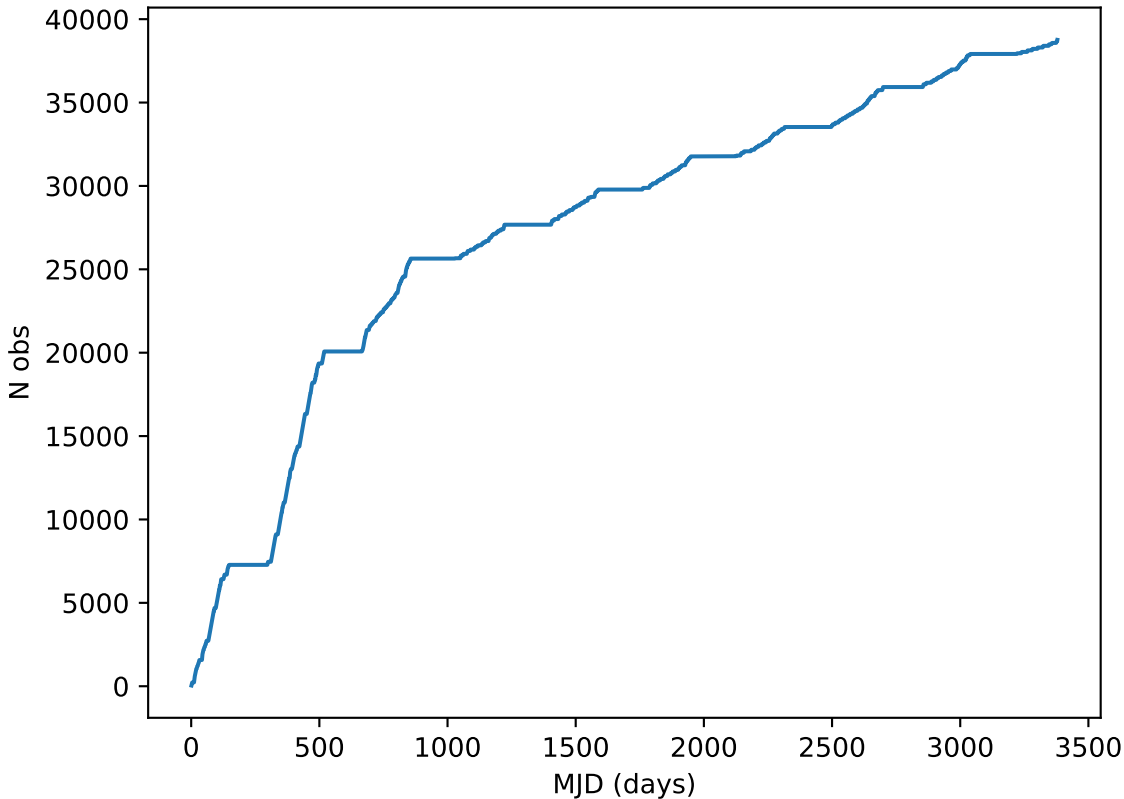
roll_pause_mjdp270_v3.4_10yrs all bands: DD: COSMOS Cumulative NVisits
