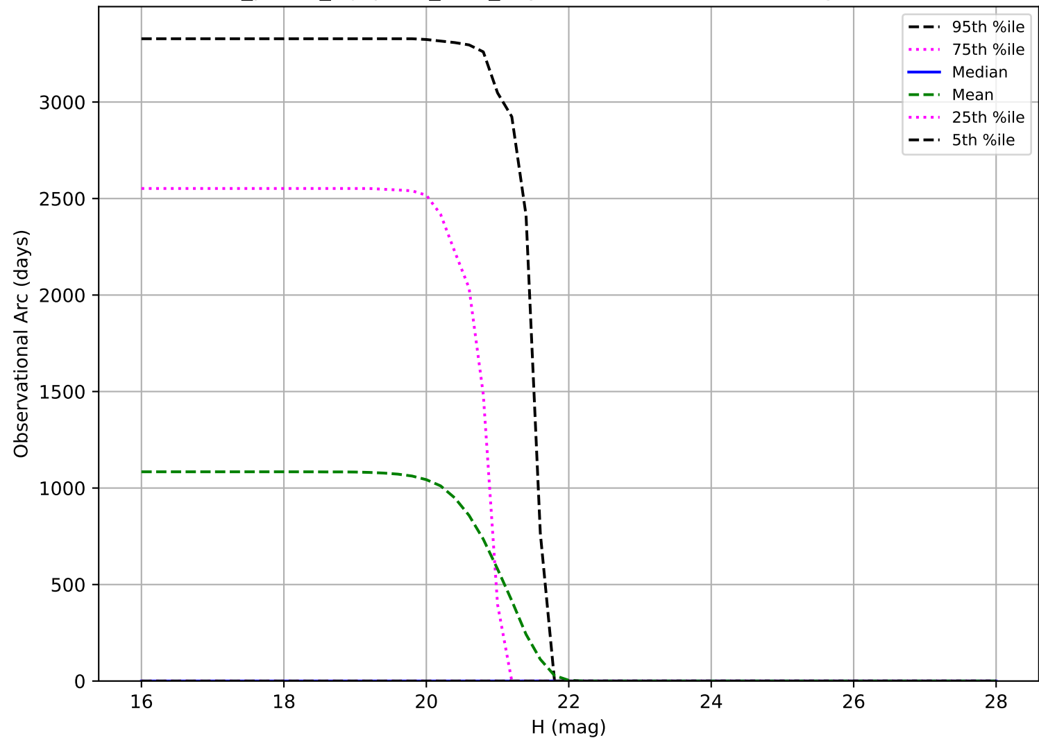
roll_pause_mjdp180_v3.4_10yrs: Observational Arc Length Vatira
