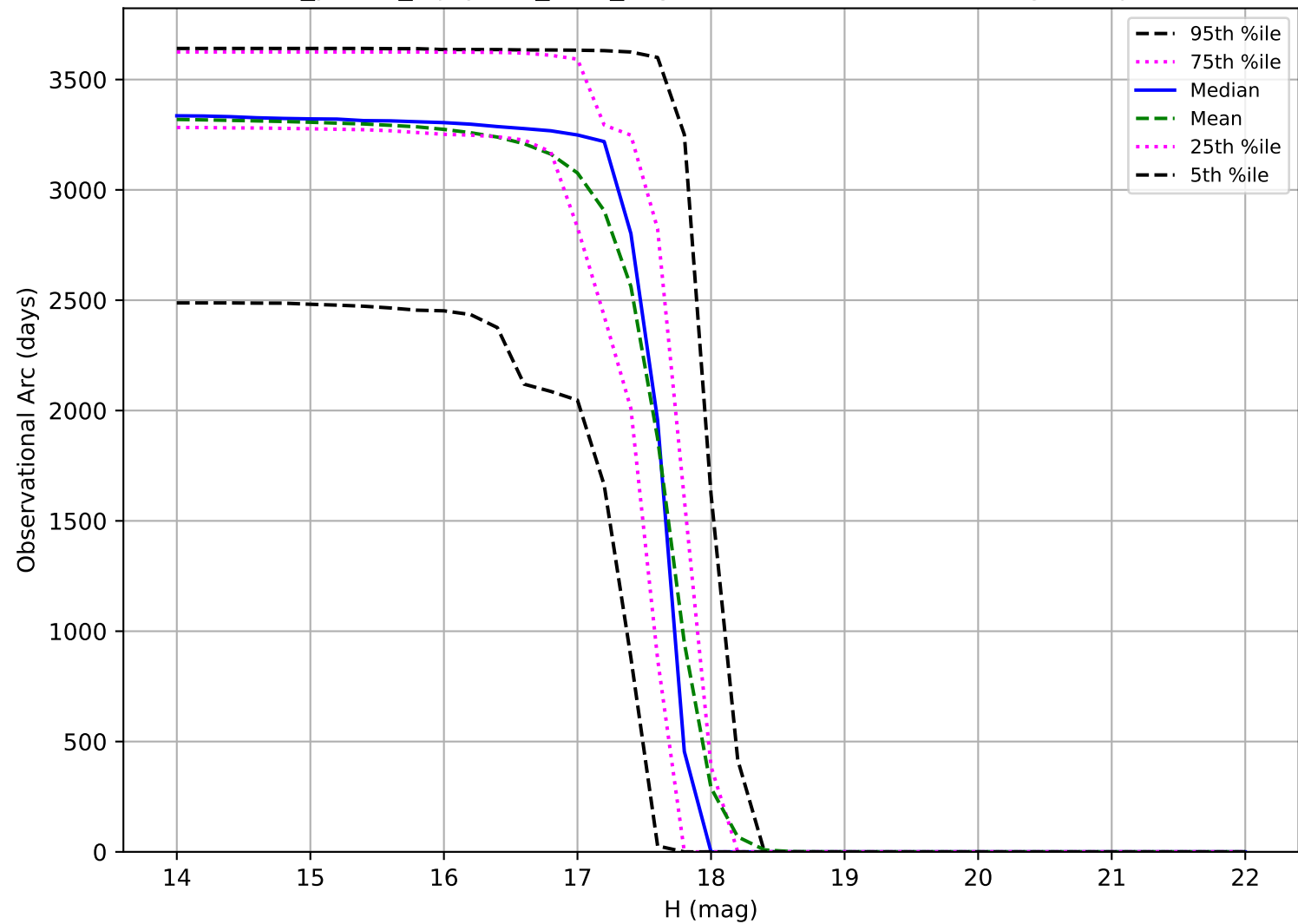
roll_pause_mjdp180_v3.4_10yrs: Observational Arc Length Trojan
