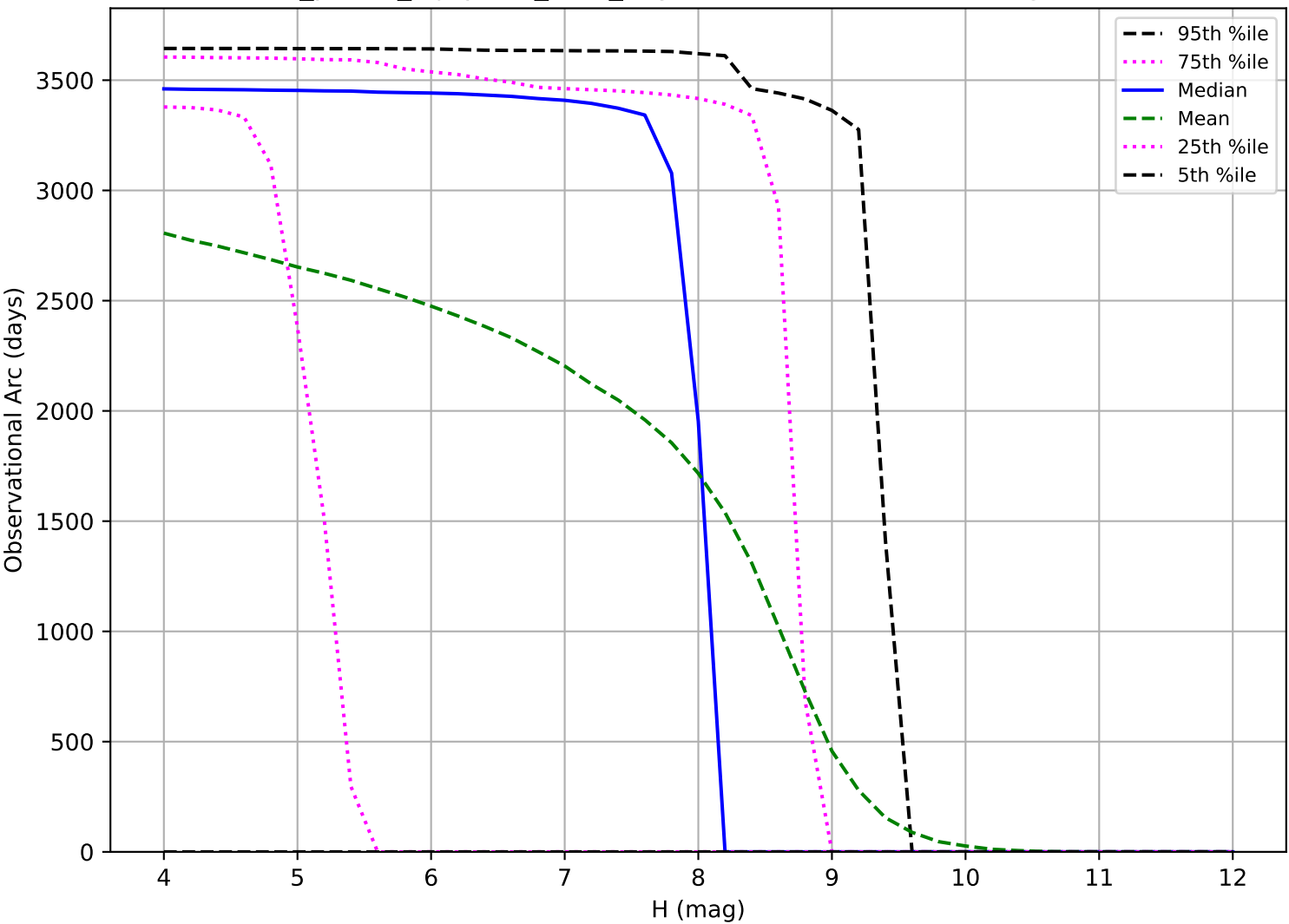
roll_pause_mjdp180_v3.4_10yrs: Observational Arc Length TNO
