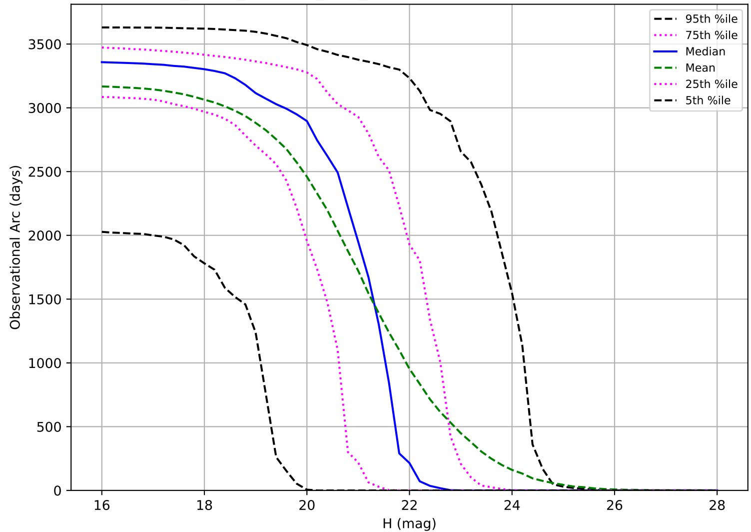
roll_pause_mjdp180_v3.4_10yrs: Observational Arc Length PHA
