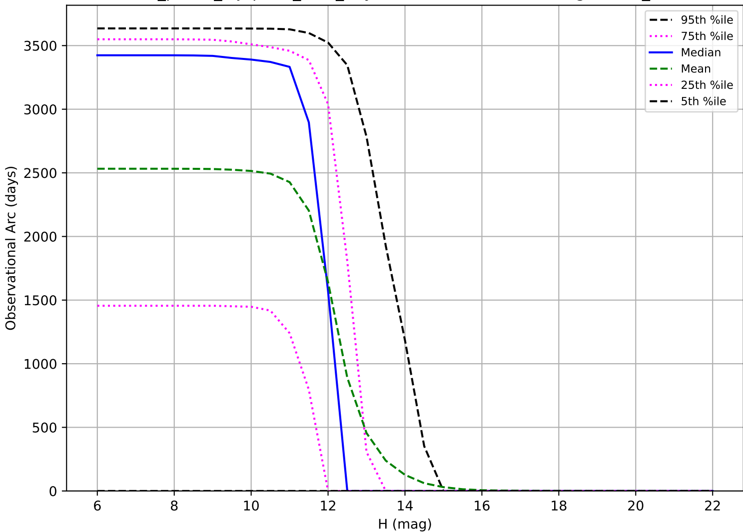
roll_pause_mjdp180_v3.4_10yrs: Observational Arc Length OCC_r20
