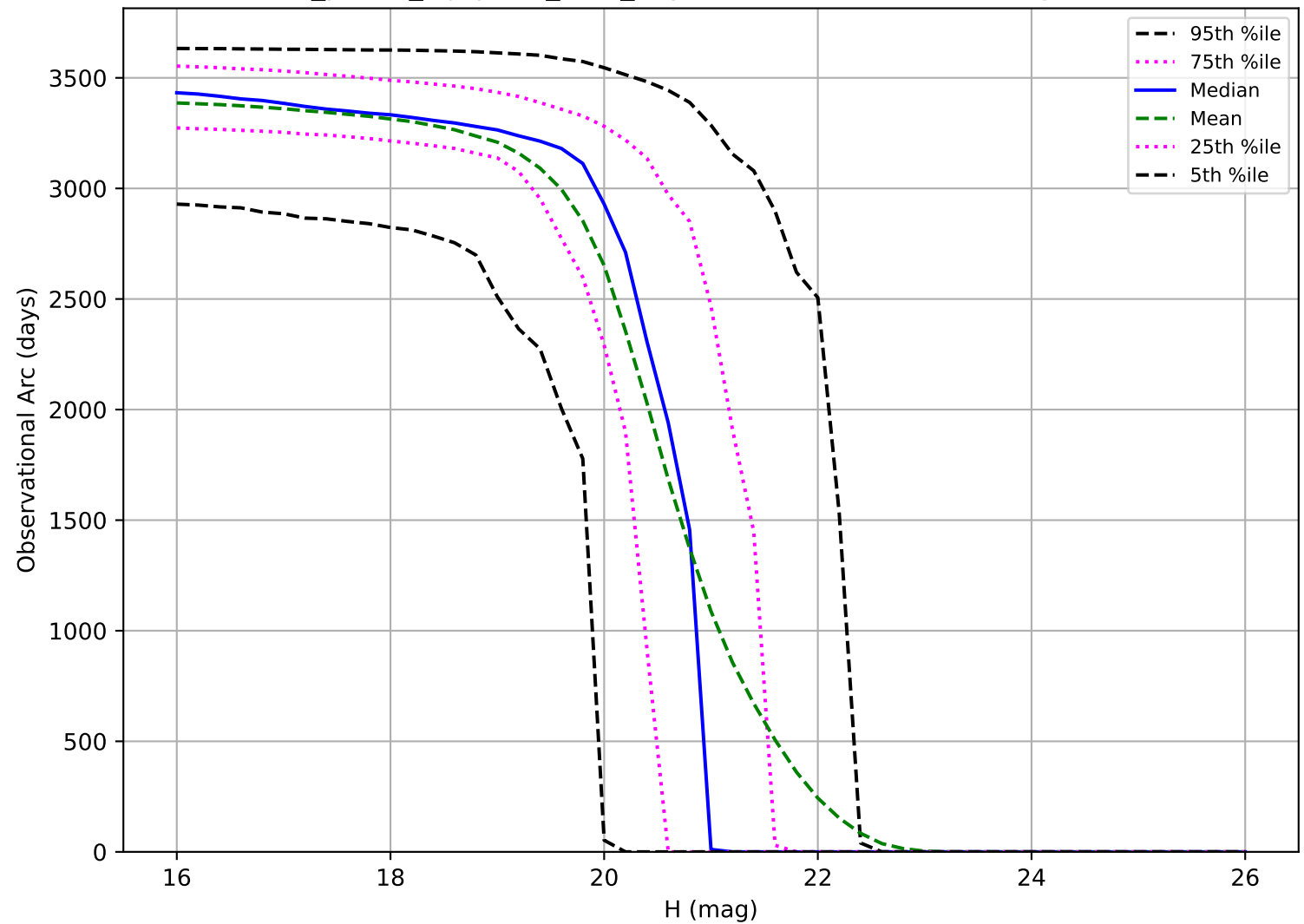
roll_pause_mjdp180_v3.4_10yrs: Observational Arc Length MBA
