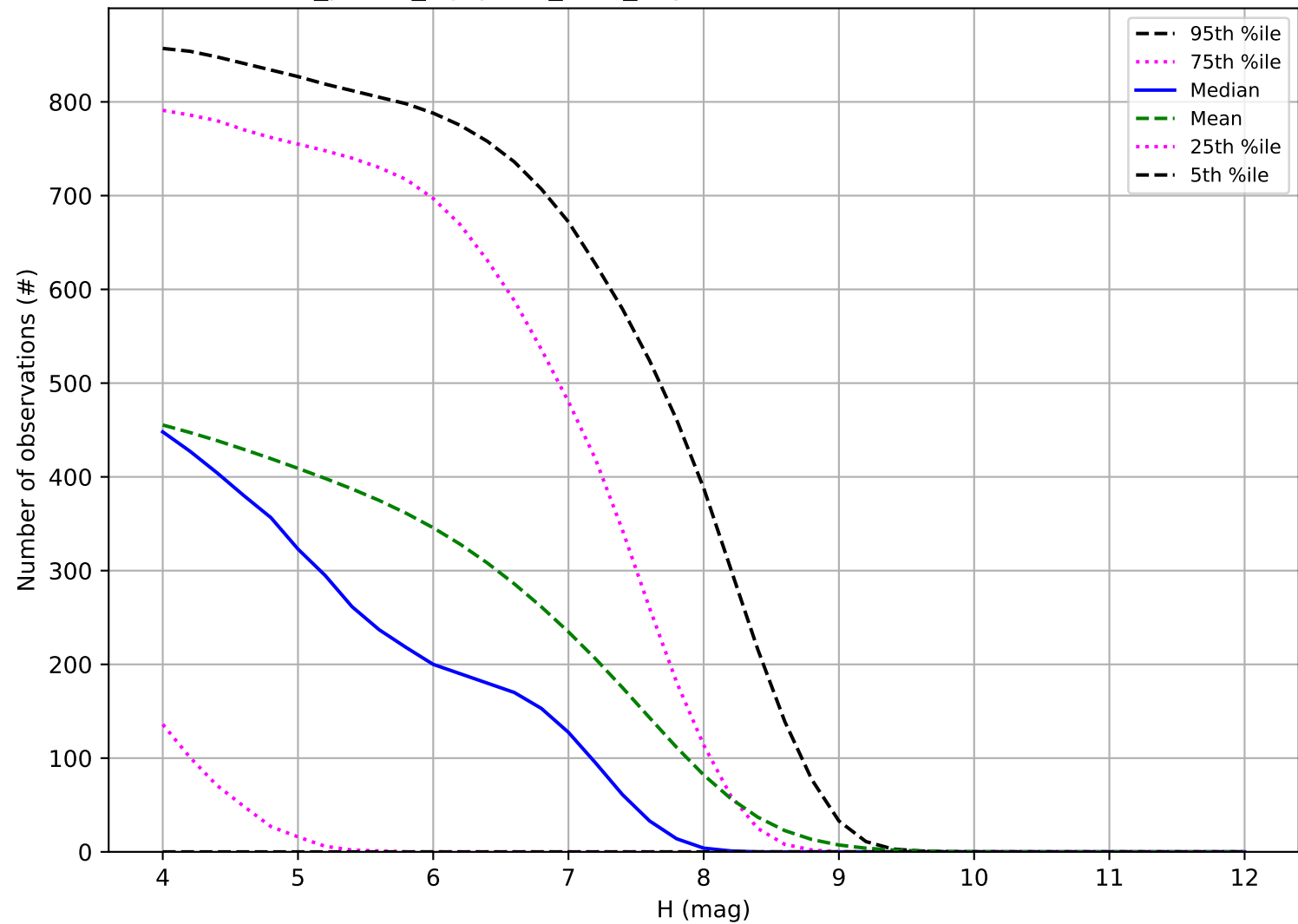
roll_pause_mjdp180_v3.4_10yrs: Number of observations TNO
