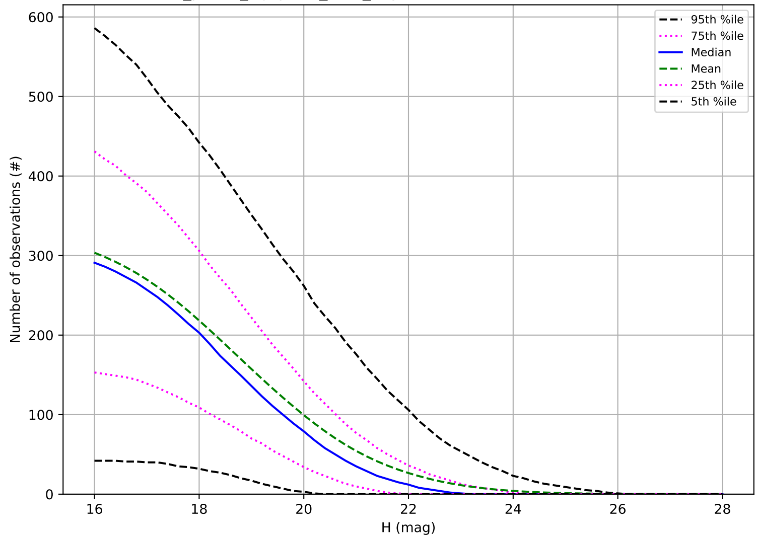
roll_pause_mjdp180_v3.4_10yrs: Number of observations PHA
