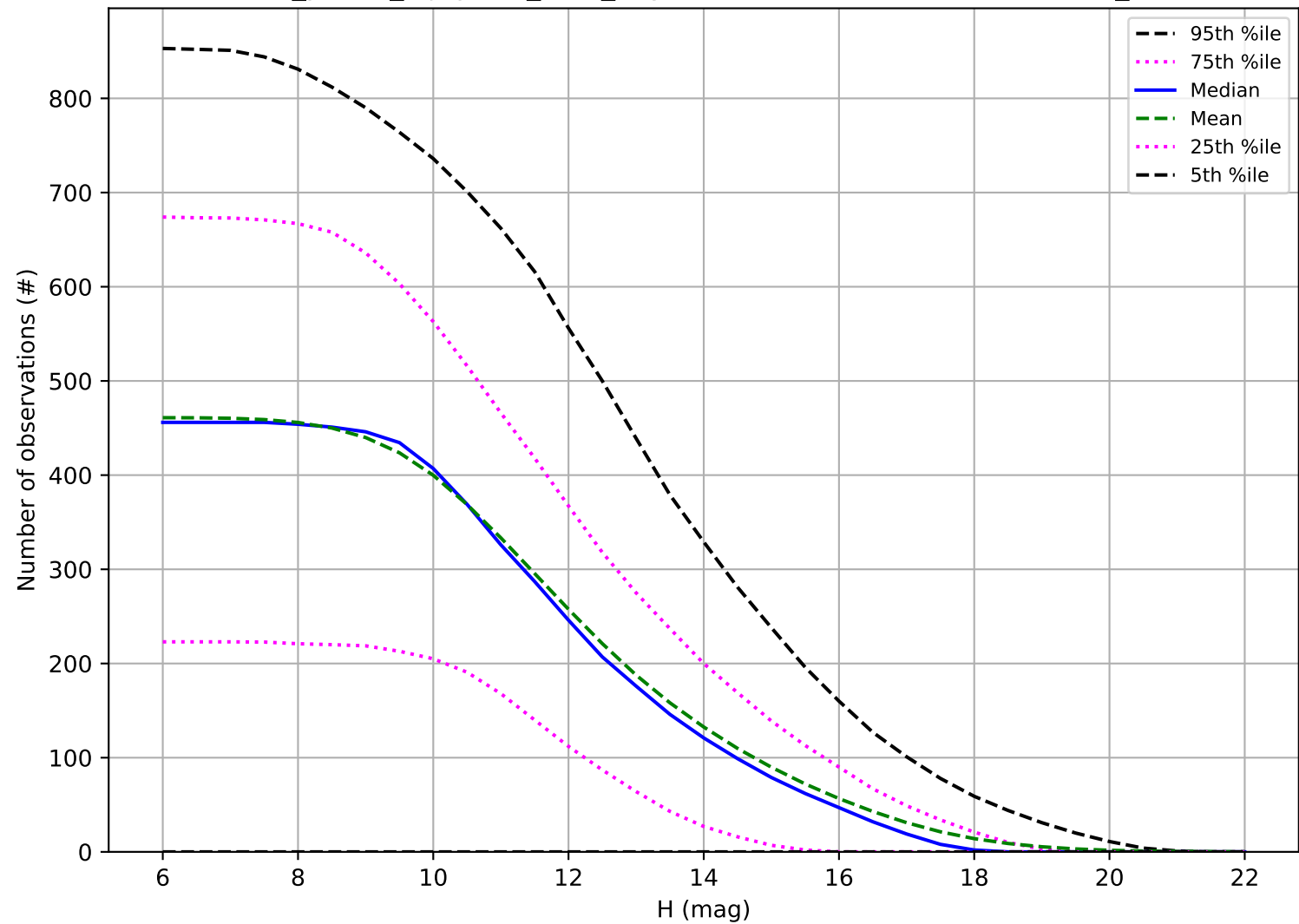
roll_pause_mjdp180_v3.4_10yrs: Number of observations OCC_r5
