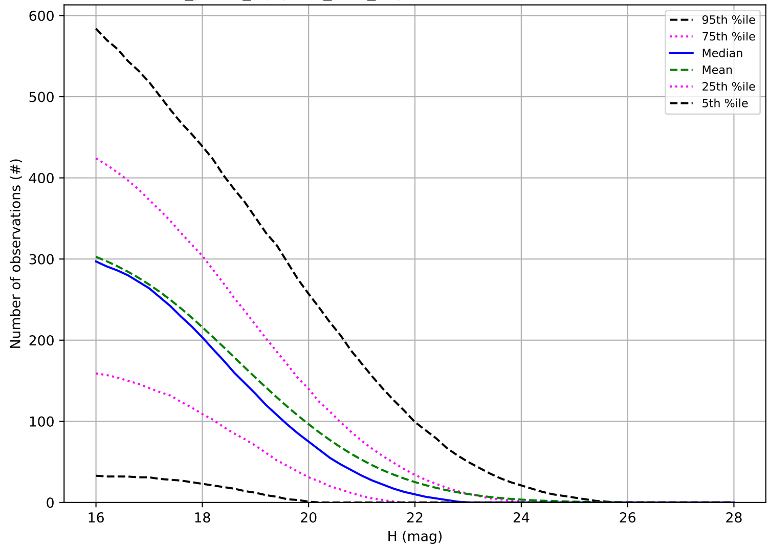
roll_pause_mjdp180_v3.4_10yrs: Number of observations NEO
