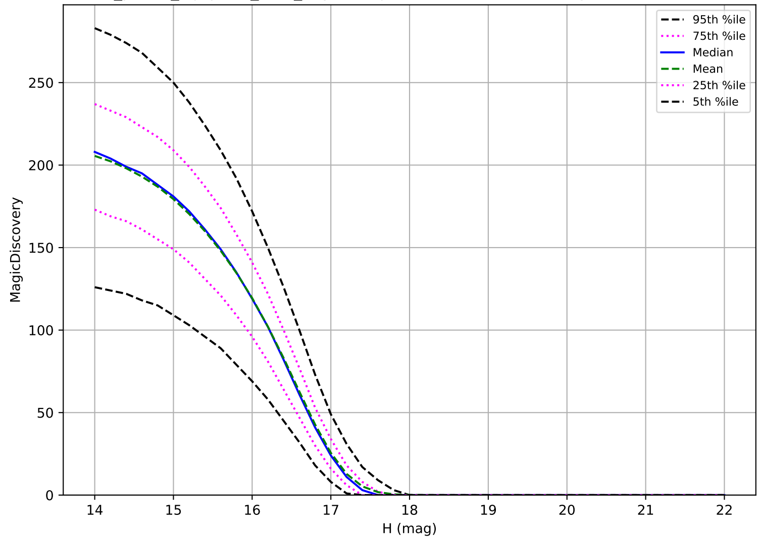
roll_pause_mjdp180_v3.4_10yrs: Trojan 6 detections in 60 nights detection loss
