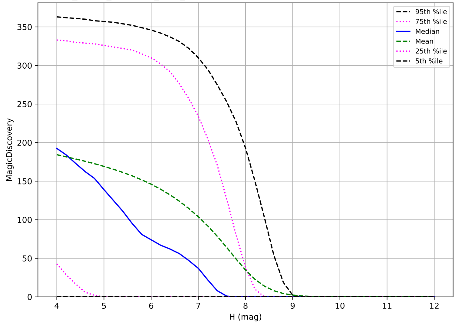
roll_pause_mjdp180_v3.4_10yrs: TNO 6 detections in 60 nights detection loss
