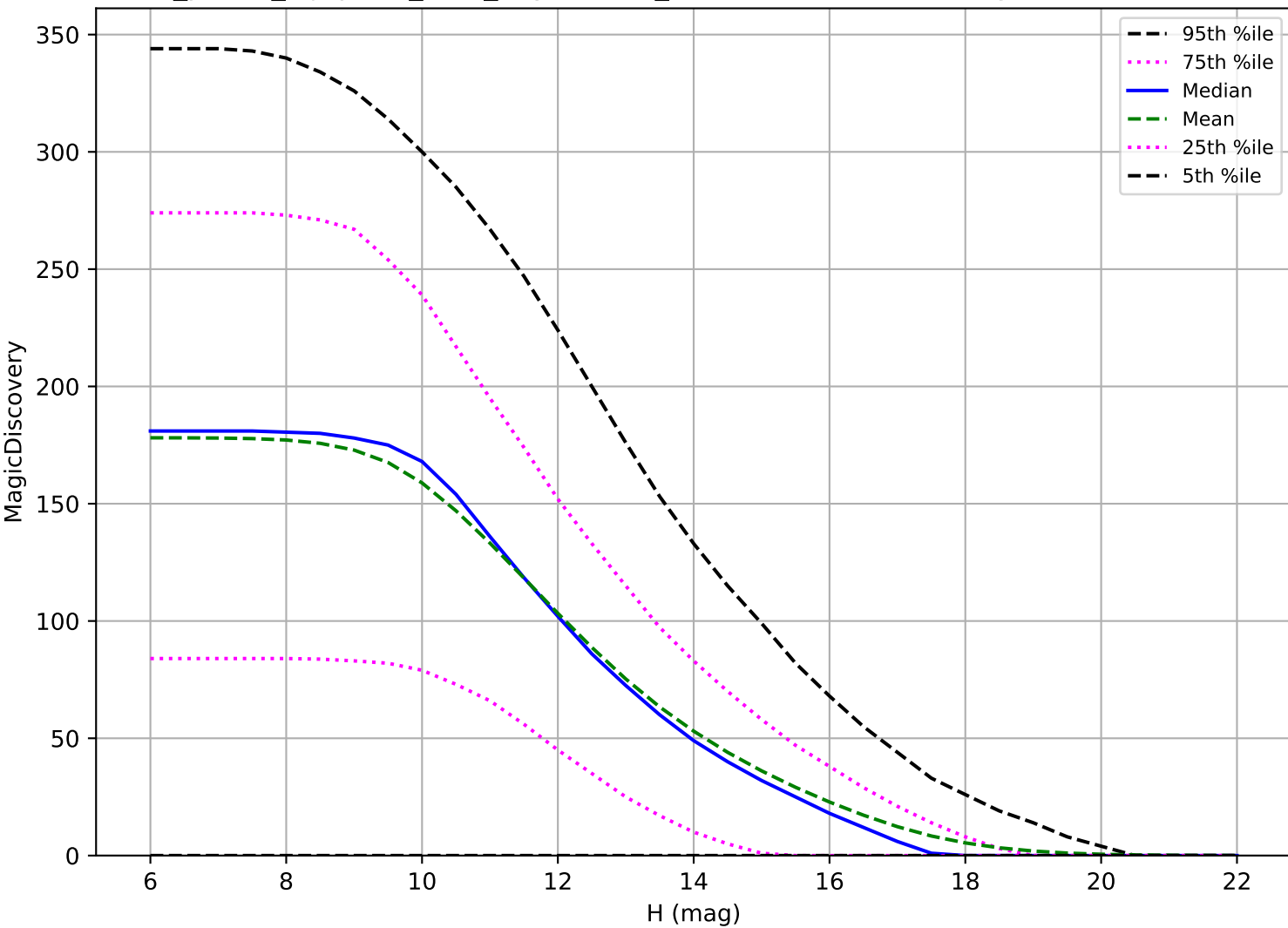
roll_pause_mjdp180_v3.4_10yrs: OCC_r5 6 detections in 60 nights detection loss
