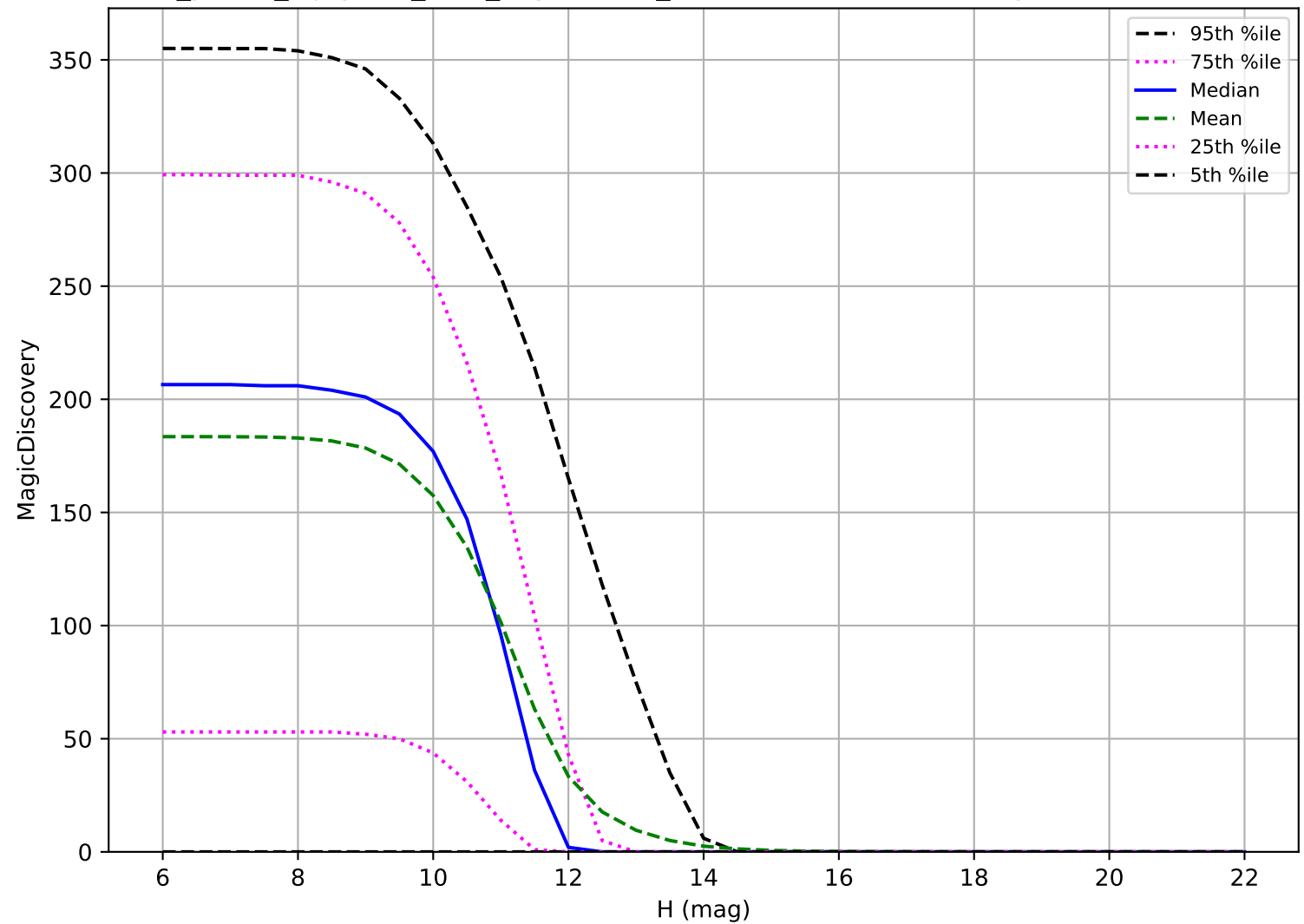
roll_pause_mjdp180_v3.4_10yrs: OCC_r20 6 detections in 60 nights detection loss
