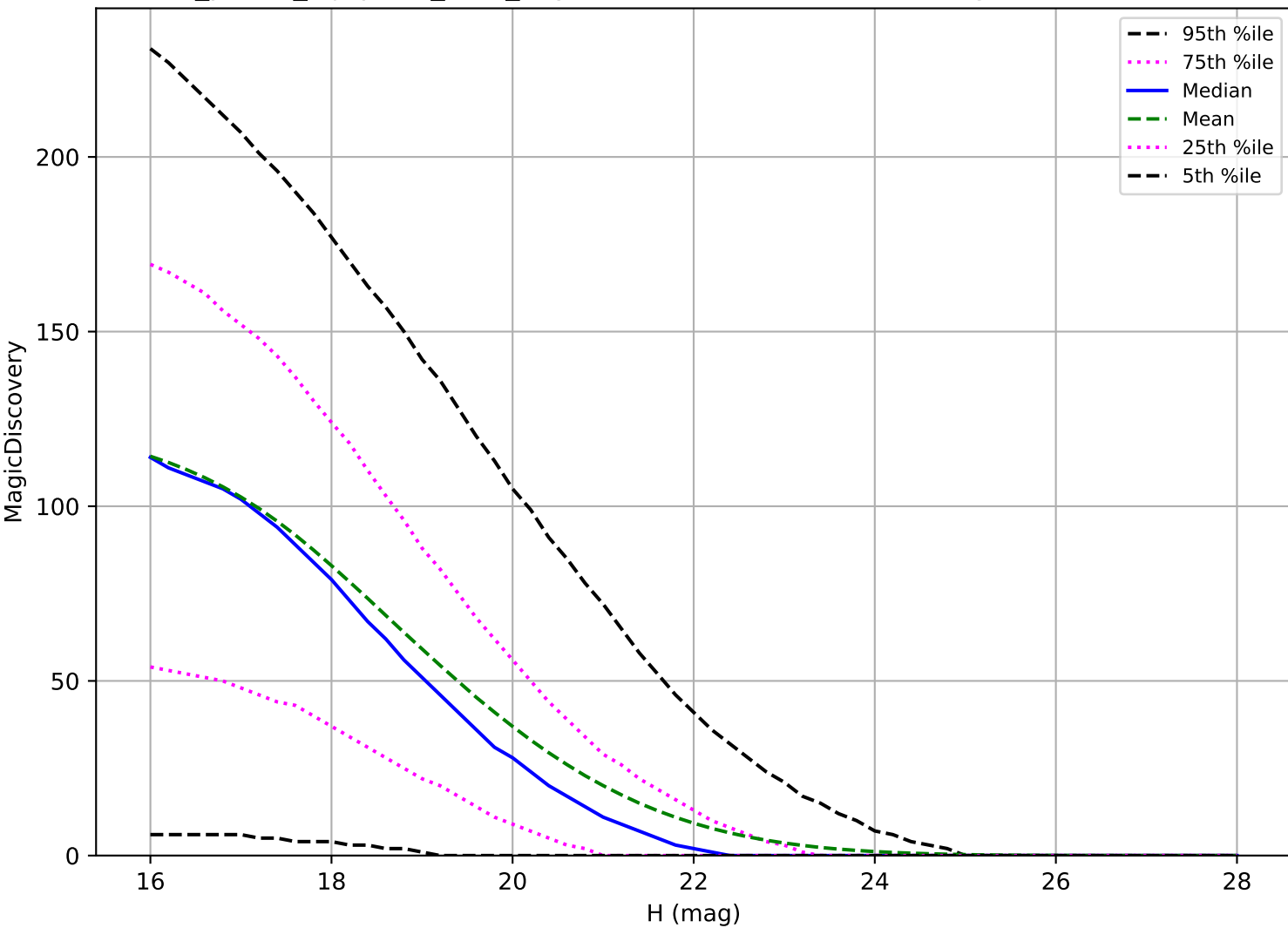
roll_pause_mjdp180_v3.4_10yrs: NEO 6 detections in 60 nights detection loss
