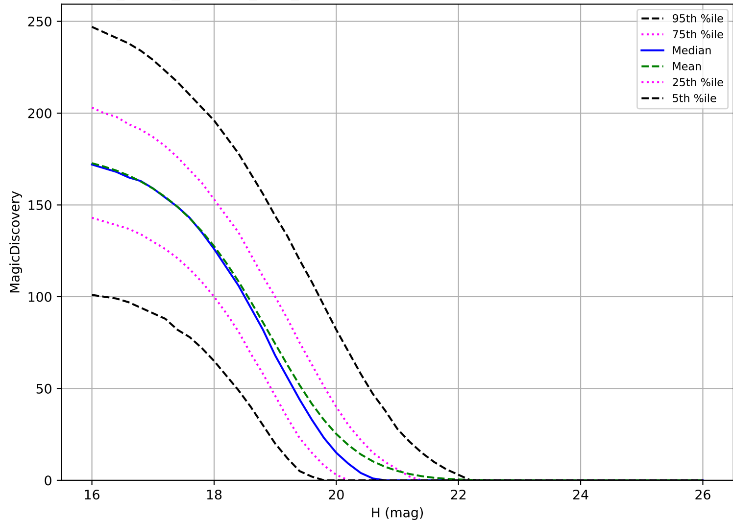
roll_pause_mjdp180_v3.4_10yrs: MBA 6 detections in 60 nights detection loss
