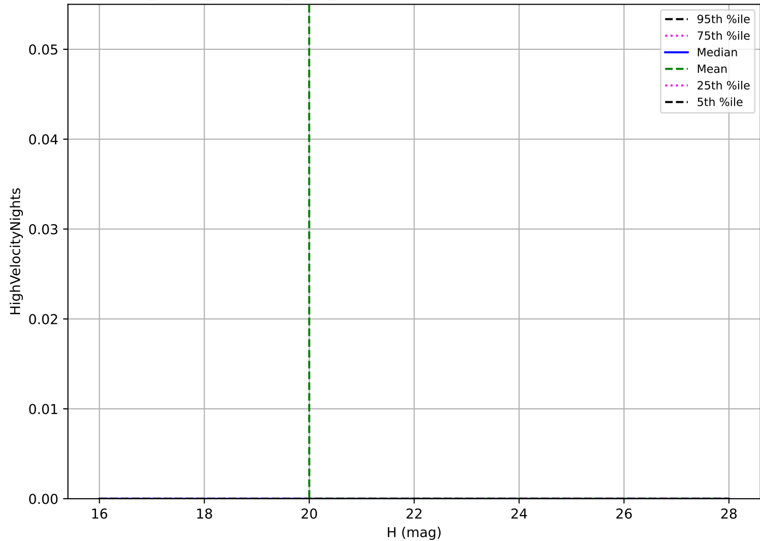
roll_pause_mjdp180_v3.4_10yrs: Vatira High velocity pair detection loss
