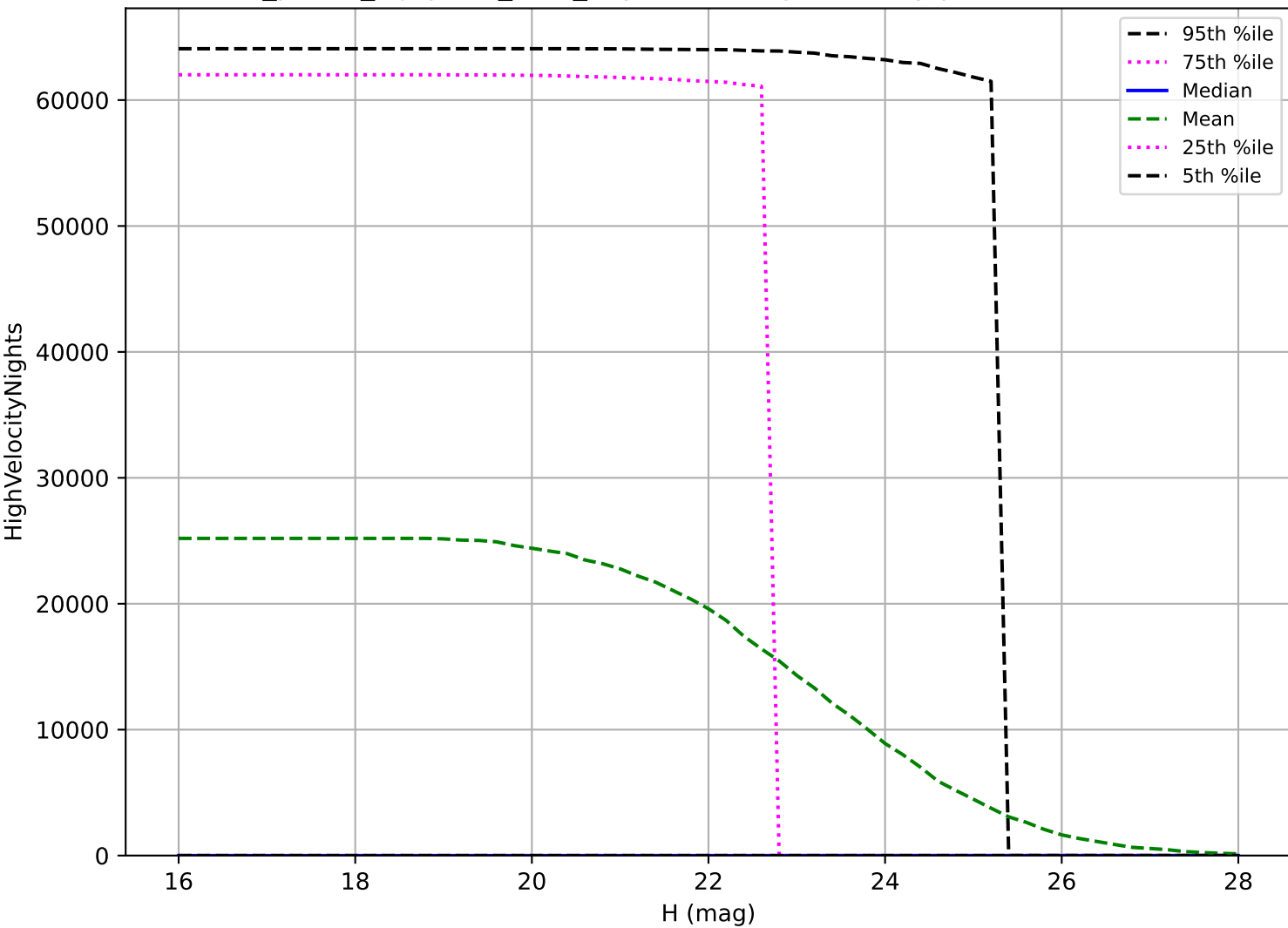
roll_pause_mjdp180_v3.4_10yrs: PHA High velocity pair detection loss
