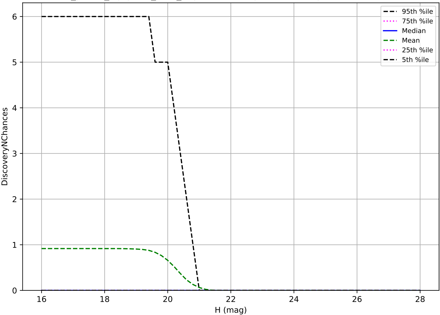
roll_pause_mjdp180_v3.4_10yrs: Vatira 3 pairs in 15 nights detection loss
