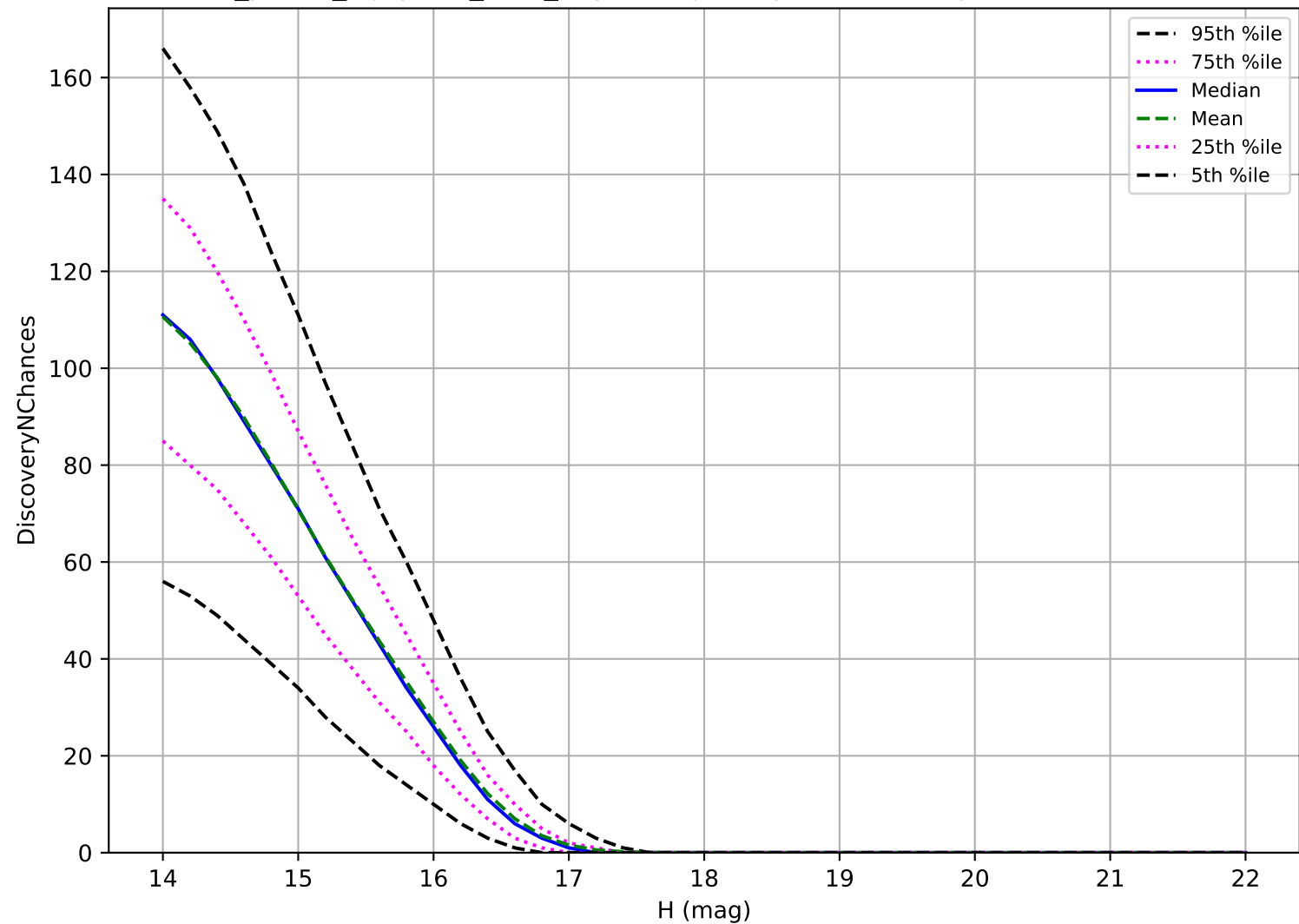
roll_pause_mjdp180_v3.4_10yrs: Trojan 3 pairs in 15 nights detection loss
