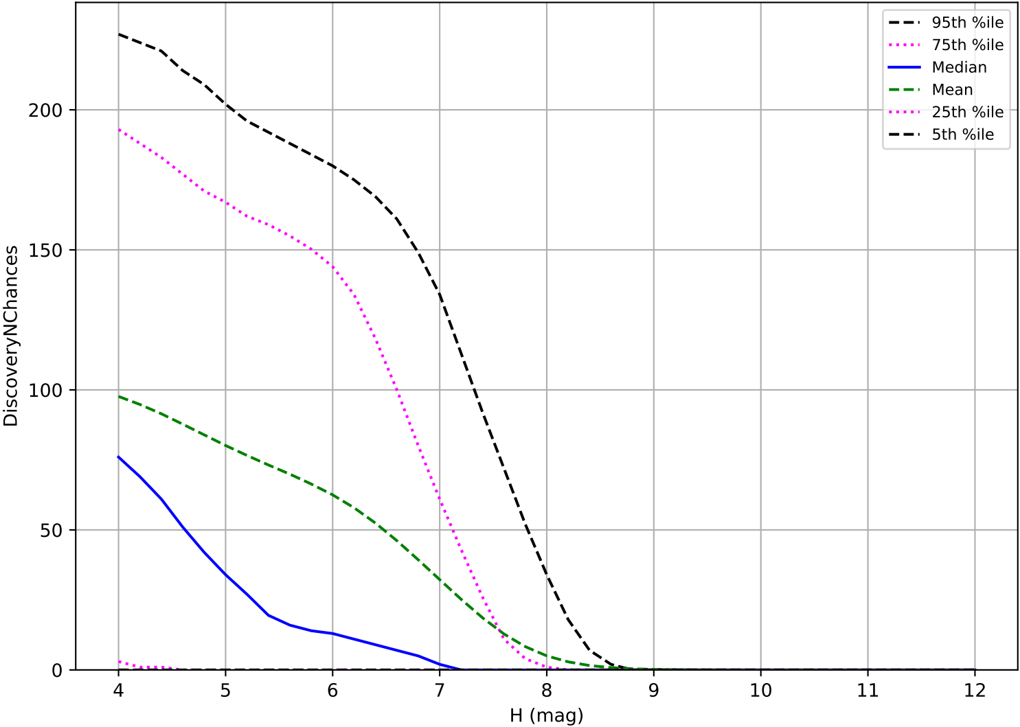
roll_pause_mjdp180_v3.4_10yrs: TNO 3 pairs in 15 nights detection loss
