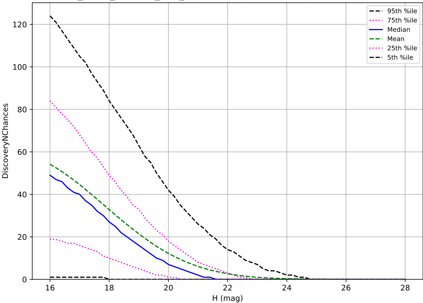
roll_pause_mjdp180_v3.4_10yrs: PHA 3 pairs in 15 nights detection loss
