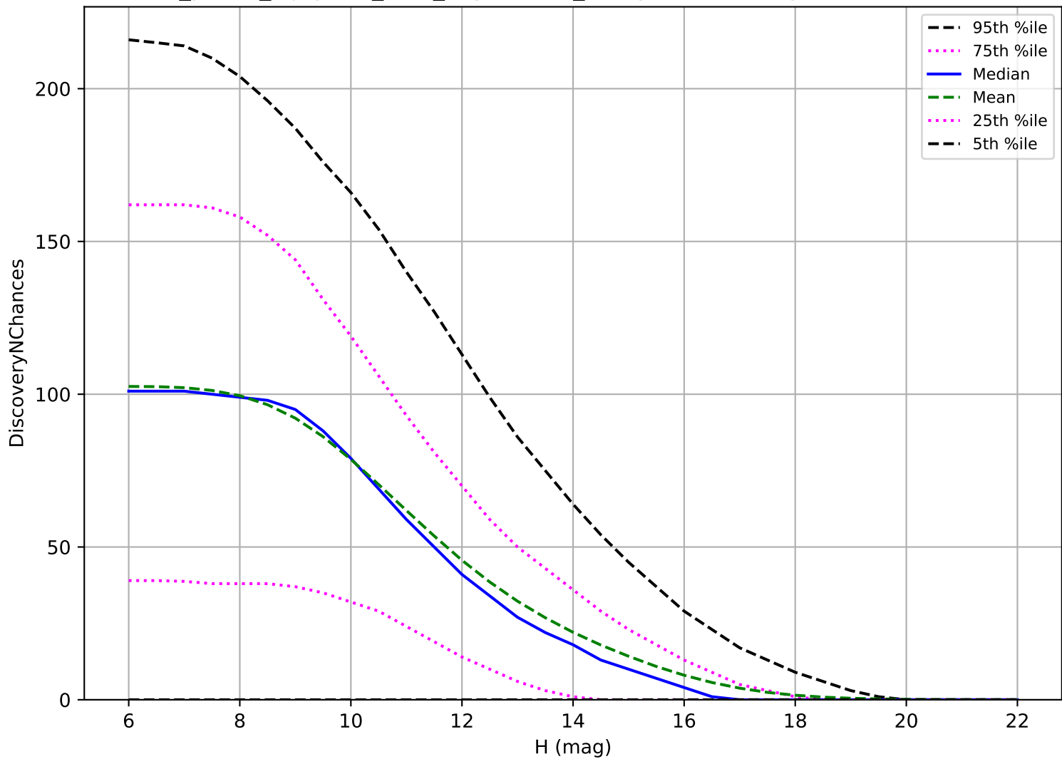
roll_pause_mjdp180_v3.4_10yrs: OCC_r5 3 pairs in 15 nights detection loss
