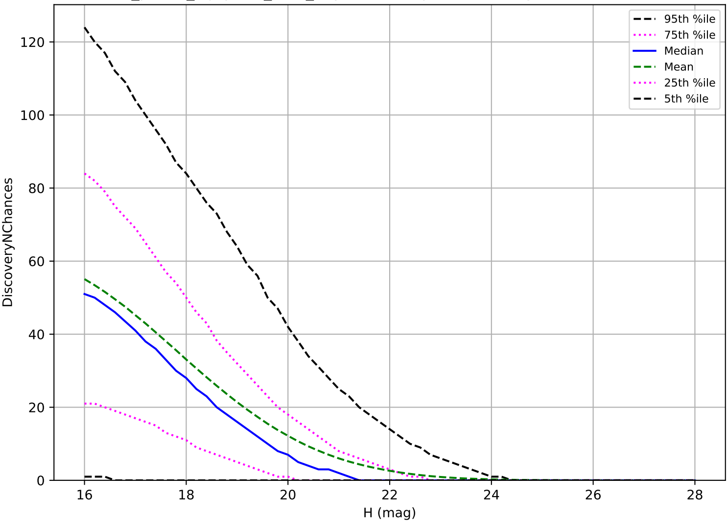
roll_pause_mjdp180_v3.4_10yrs: NEO 3 pairs in 15 nights detection loss
