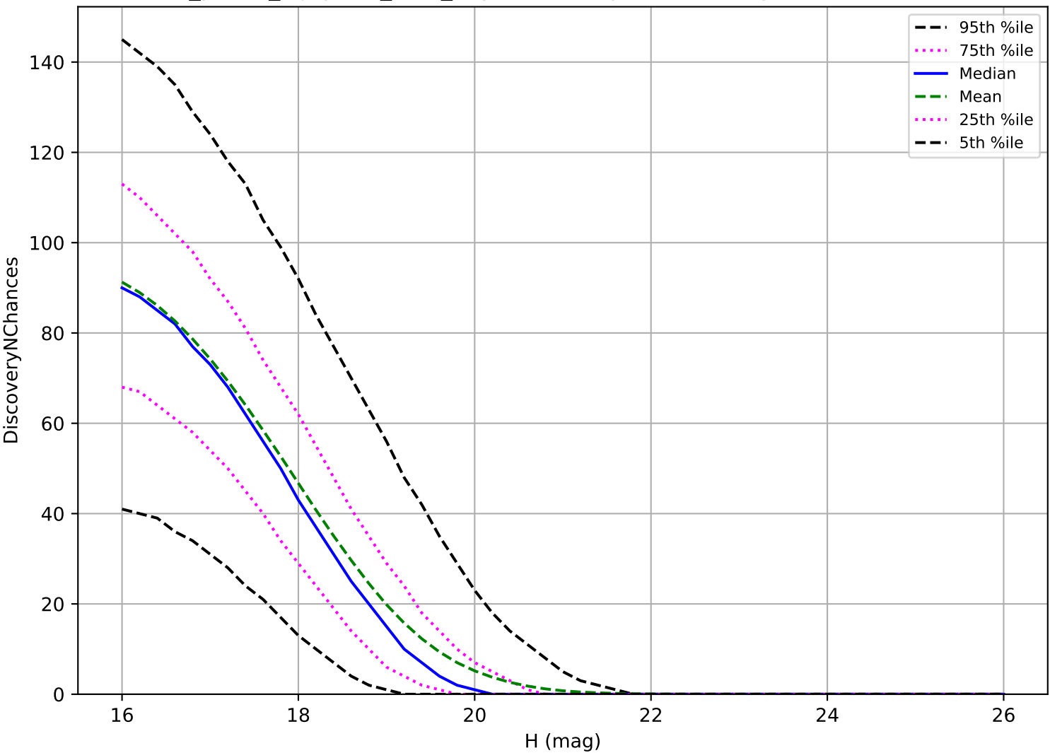
roll_pause_mjdp180_v3.4_10yrs: MBA 3 pairs in 15 nights detection loss
