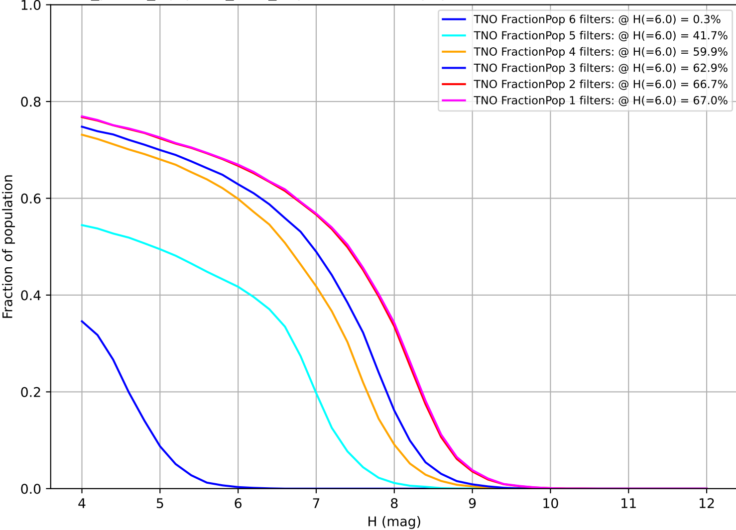
roll_pause_mjdp180_v3.4_10yrs: Fraction of population with colors in X filters TNO
