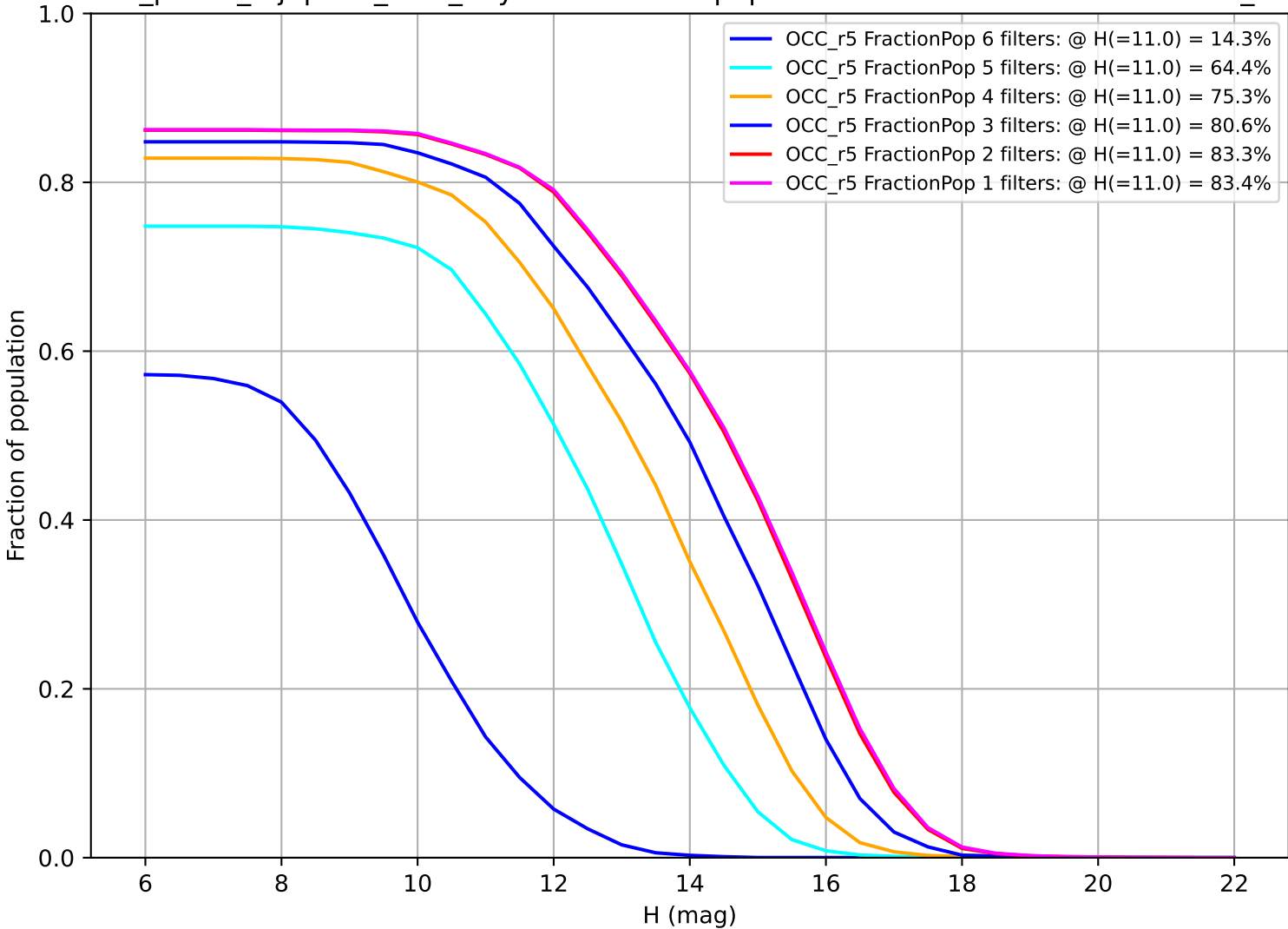
roll_pause_mjdp180_v3.4_10yrs: Fraction of population with colors in X filters OCC_r5
