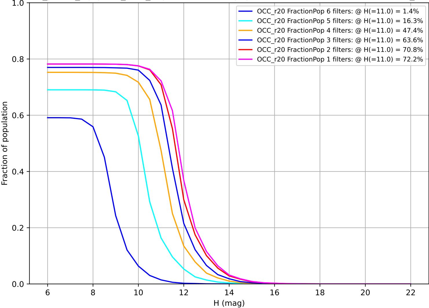
roll_pause_mjdp180_v3.4_10yrs: Fraction of population with colors in X filters OCC_r20
