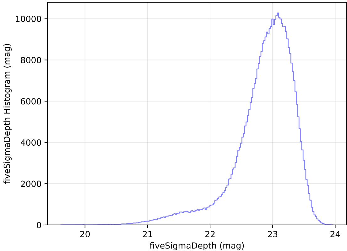
roll_pause_mjdp180_v3.4_10yrs z: fiveSigmaDepth Histogram
