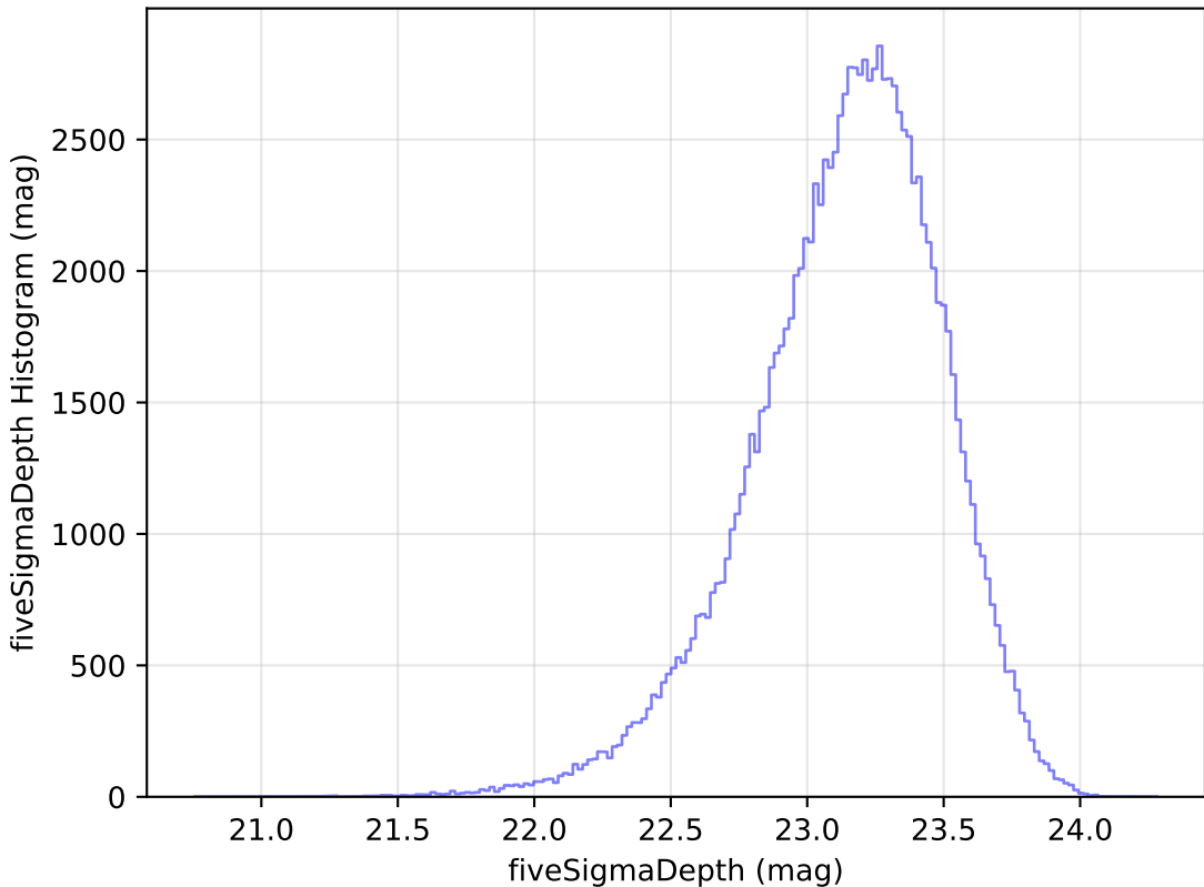
roll_pause_mjdp180_v3.4_10yrs u: fiveSigmaDepth Histogram
