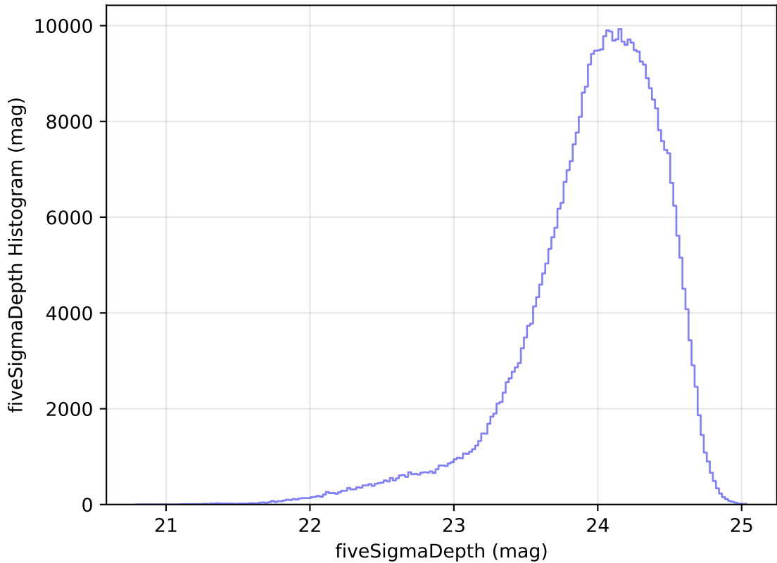
roll_pause_mjdp180_v3.4_10yrs r: fiveSigmaDepth Histogram
