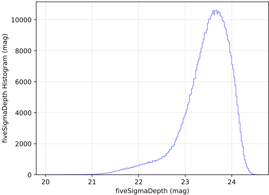
roll_pause_mjdp180_v3.4_10yrs i: fiveSigmaDepth Histogram
