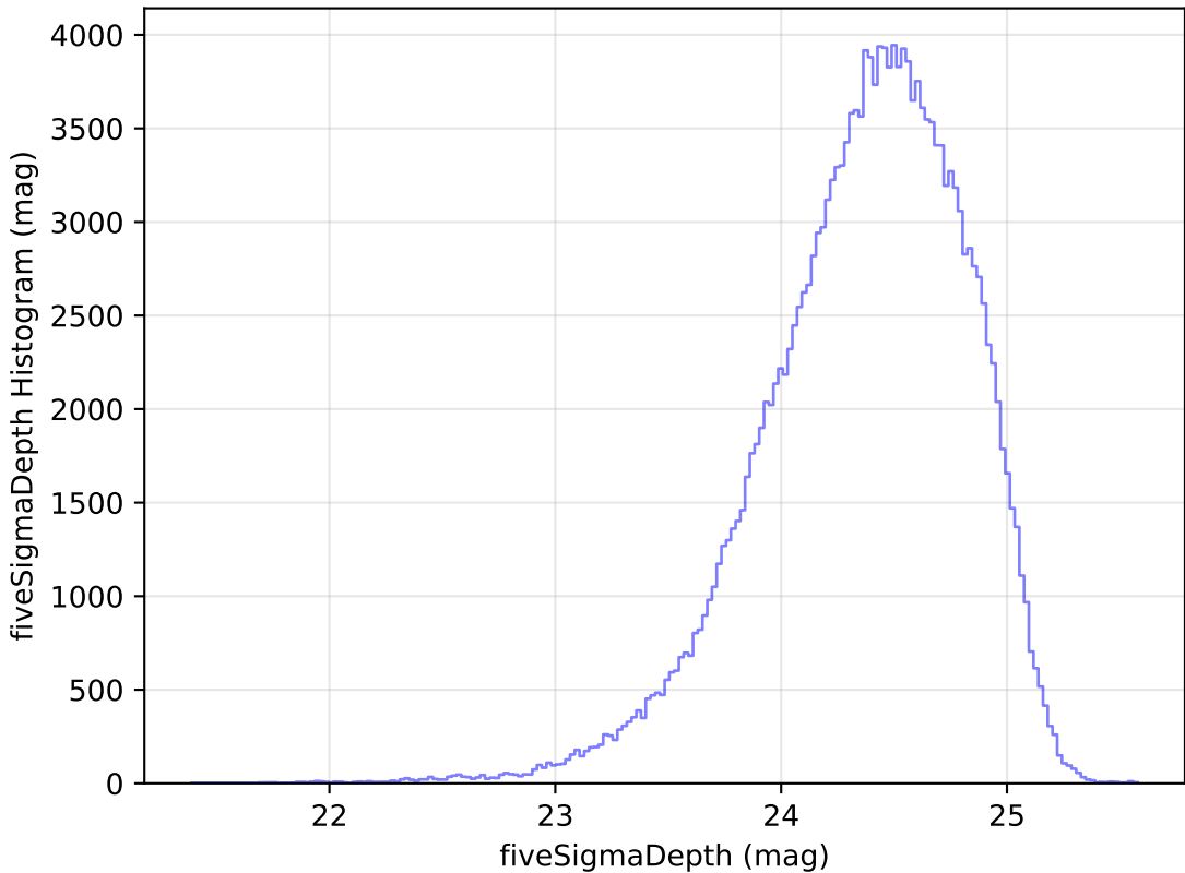
roll_pause_mjdp180_v3.4_10yrs g: fiveSigmaDepth Histogram
