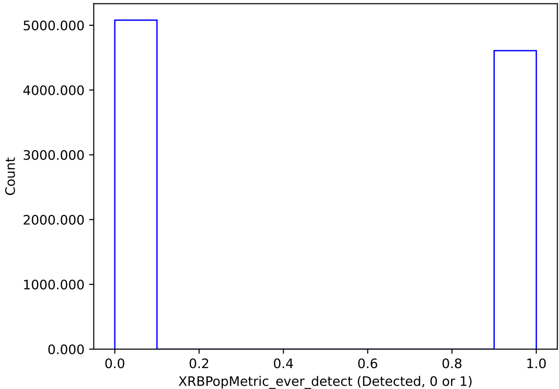
roll_pause_mjdp180_v3.4_10yrs : XRBPoMetric_ever_detect
